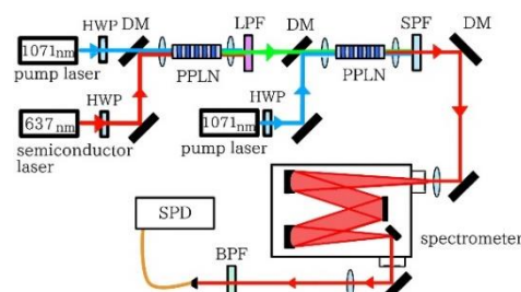
Fig 1. 実験装置 (LPF: long pass filter、SPF: short pass filter、BPF: bandpass filter、DM: dichroic mirror、HWP: half-wave plate、SPD: single photon detector)
